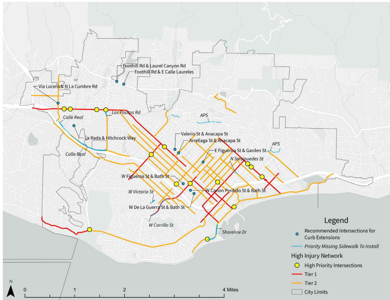
Figure 7: Additional Intersection Safety Enhancements and Sidewalk Infill.
