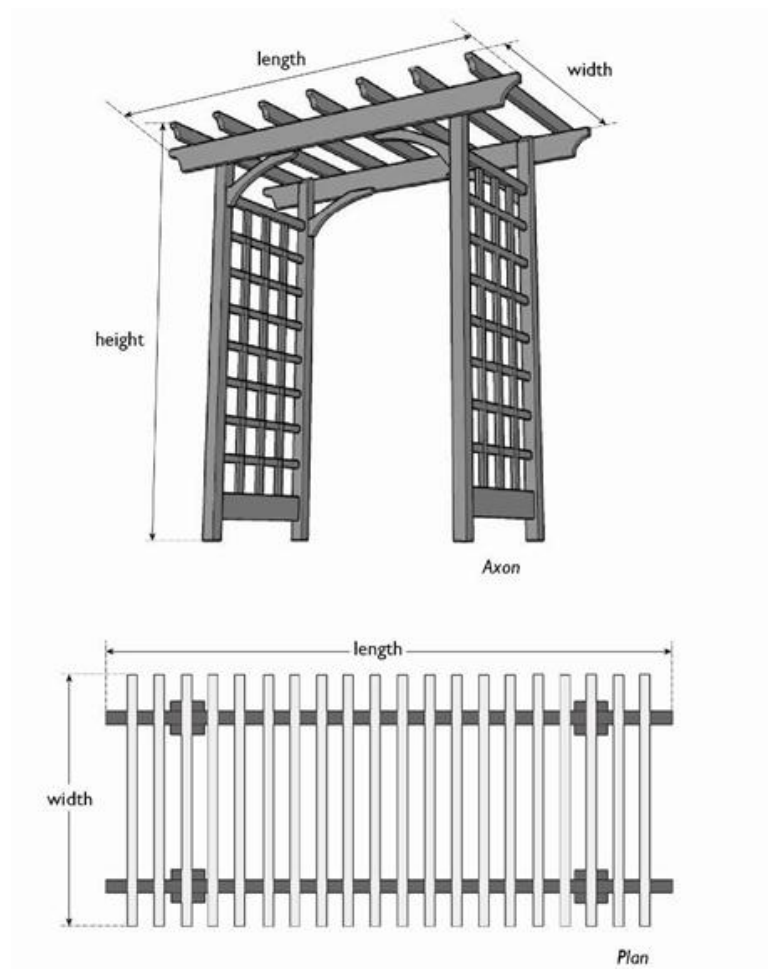
FIGURE 30.300.200: TRELLIS
