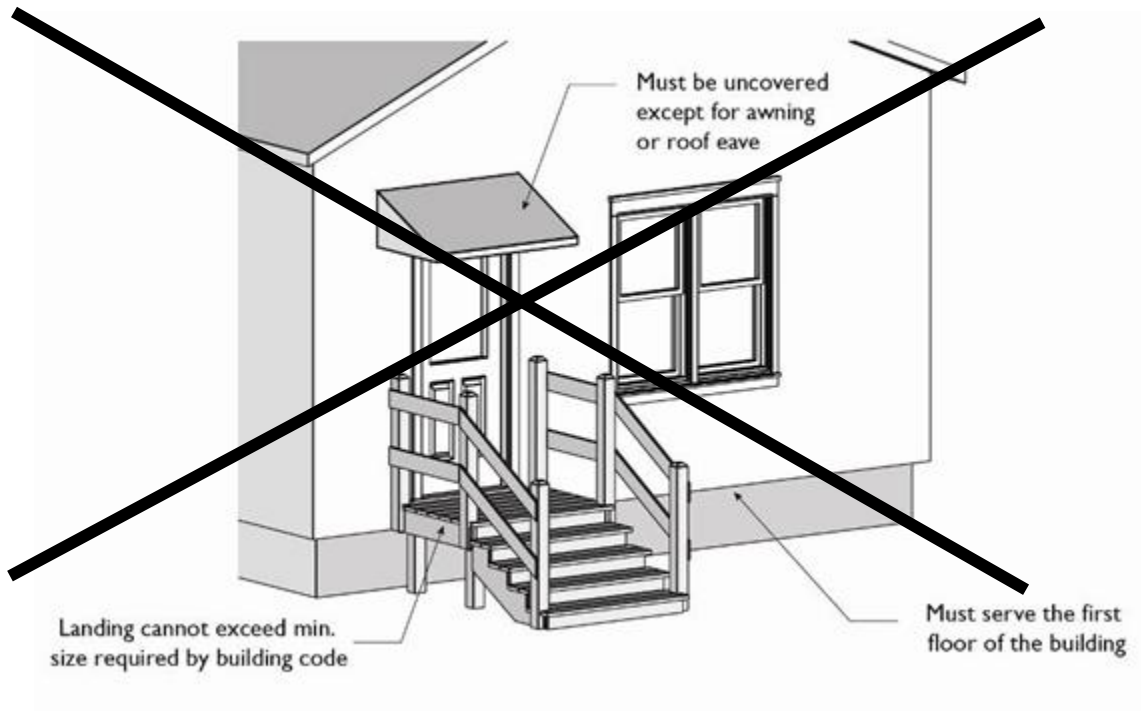
FIGURE 30.140.090.C-6: STOOPS, LANDINGS, AND OUTSIDE STEPS ENCROACHMENTS
