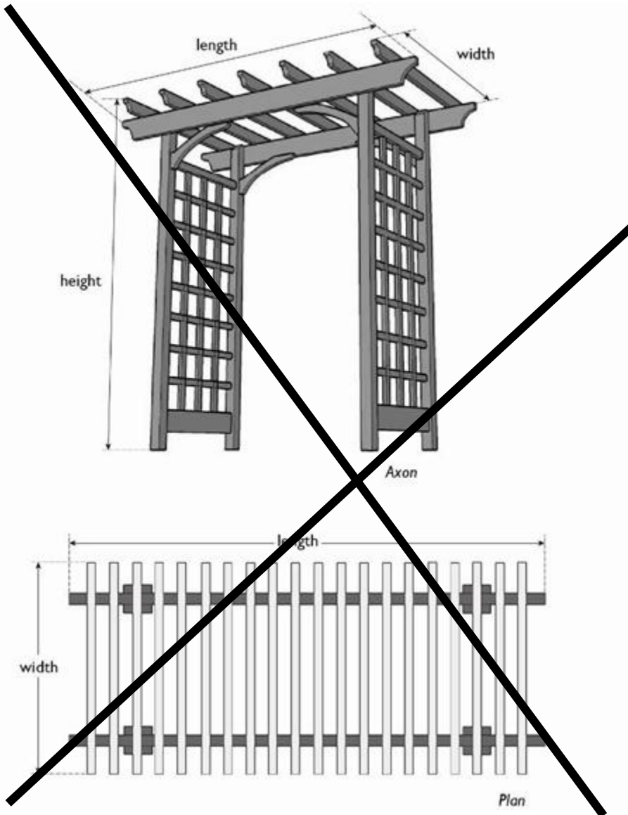
FIGURE 30.140.090.C.11: TRELLIS ENCROACHMENTS
