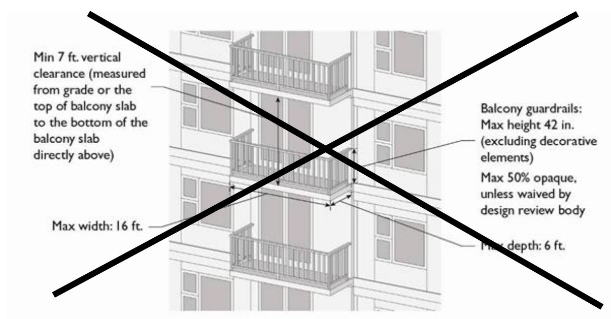
FIGURE 30.140.090.C.2: BALCONY AND UPPER STORY DECK ENCROACHMENTS
