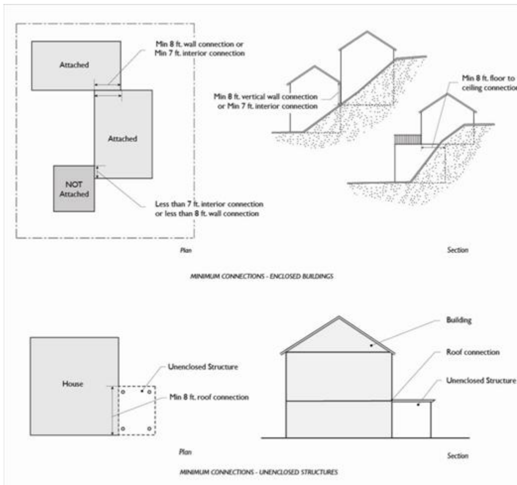
FIGURE 30.140.030: BUILDING ATTACHMENT
