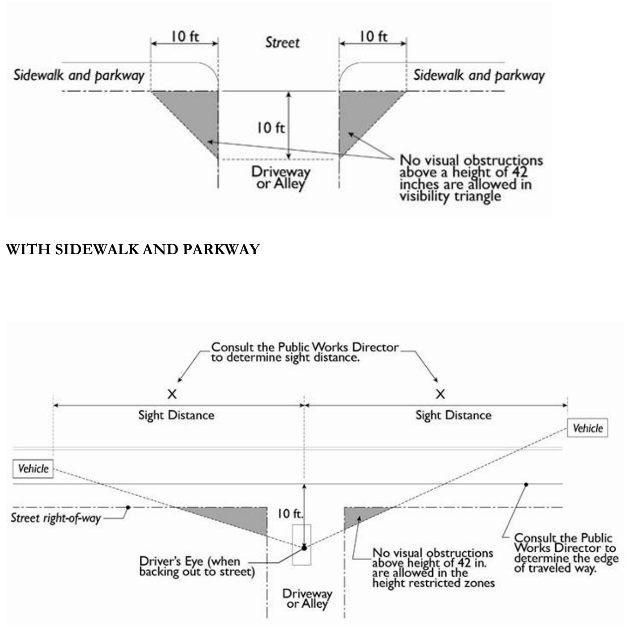
FIGURE 30.140.230: VISIBILITY AT DRIVEWAYS AND INTERSECTIONS
