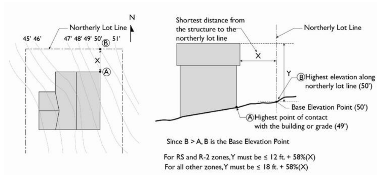
FIGURE 30.140.170: SOLAR ACCESS HEIGHT LIMITATIONS
