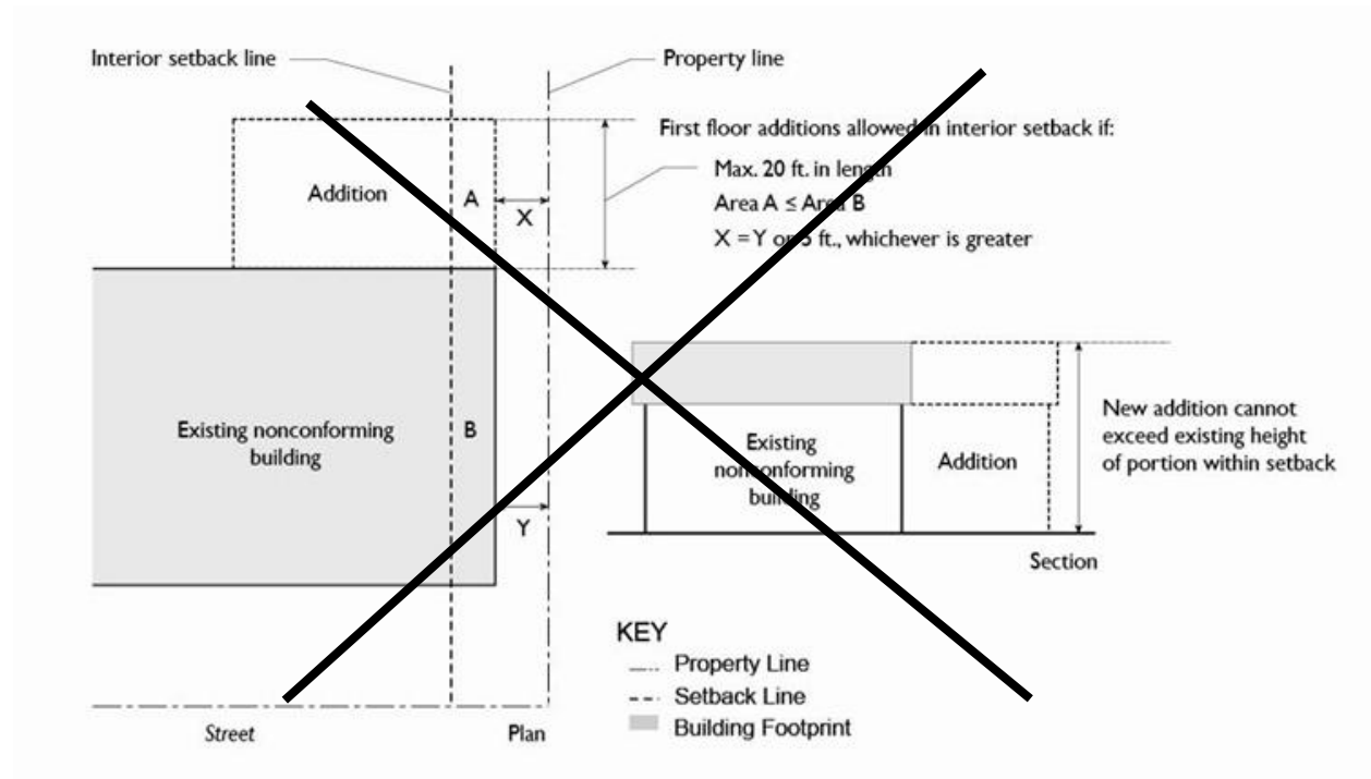
FIGURE 30.165.050.C.2: FIRST FLOOR ADDITION IN INTERIOR SETBACK
