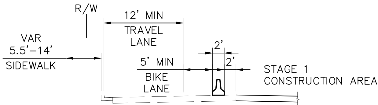
SECTION A
