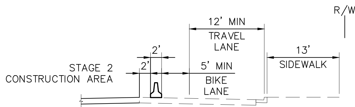
SECTION B
