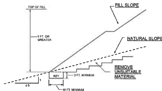
FIGURE J107.2 BENCHING DETAILS
